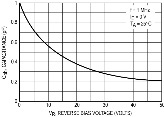
Figure 29. Output Capacitance
