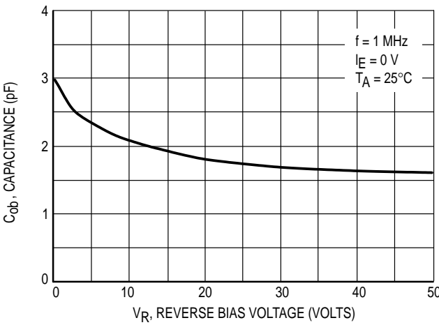
Figure 19. Output Capacitance
