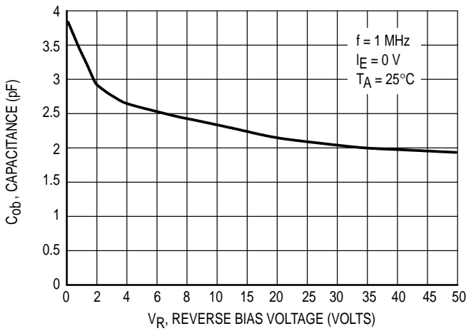
Figure 34. Output Capacitance
