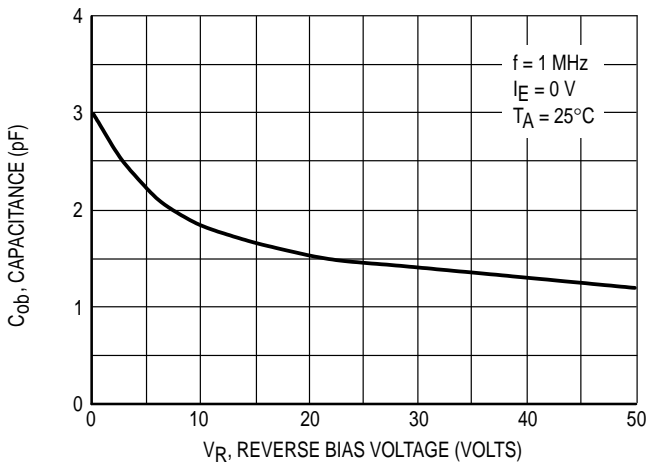
Figure 14. Output Capacitance
