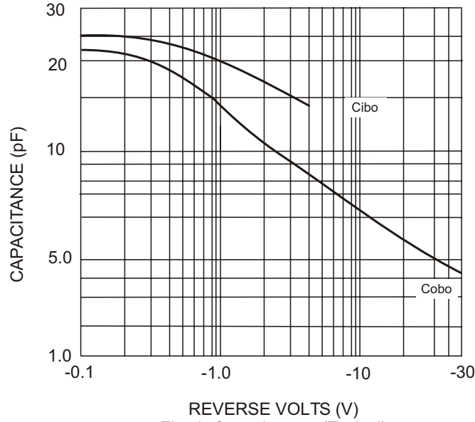
Fig. 1 Capacitances (Typical)
