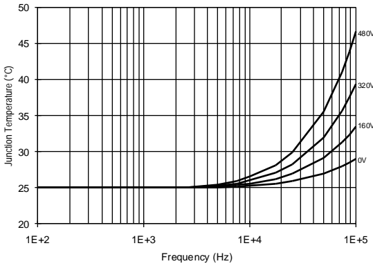
Figure 50. IR2130 T J vs. Frequency (IRF820) R GATE = 33Ω, V CC = 15V
