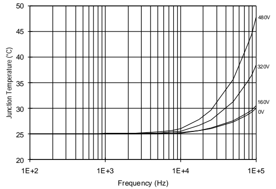
Figure 51. IR2130 T J vs. Frequency (IRF830) R GATE = 20Ω, V CC = 15V
