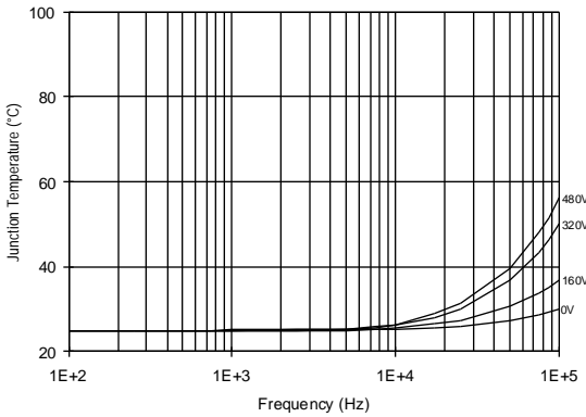
Figure 52. IR2130 T J vs. Frequency (IRF840) R GATE = 15Ω, V CC = 15V
