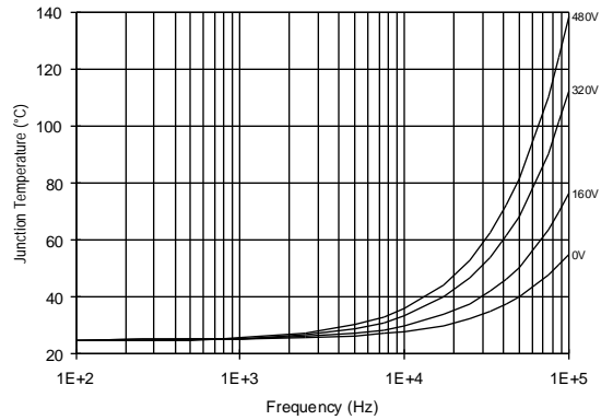
Figure 53. IR2130 T J vs. Frequency (IRF450) R GATE = 10Ω, V CC = 15V
