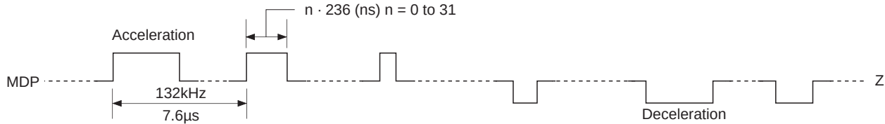
Timing Chart 1-7
