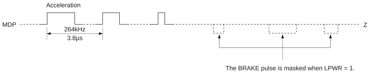
Timing Chart 1-10
