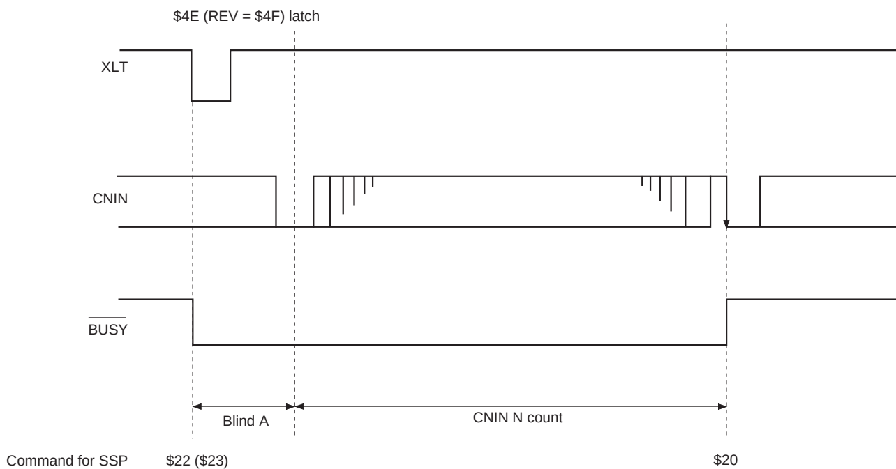
Fig. 4-7-(b). N-Track Move Timing Chart
