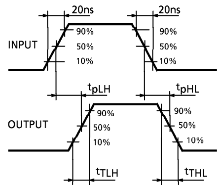
WAVEFORM
