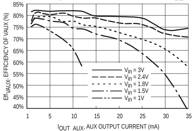
Figure 12. Efficiency of VAUX versus Output Current (VAUX = 5 V, L2 = 82 \mu H, Various V_{IN} )
