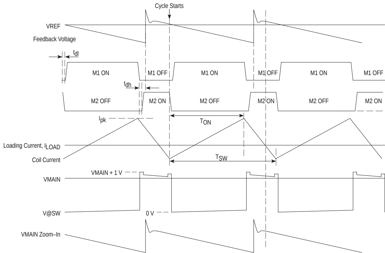
Figure 21. Waveforms of Continuous Conduction Mode
