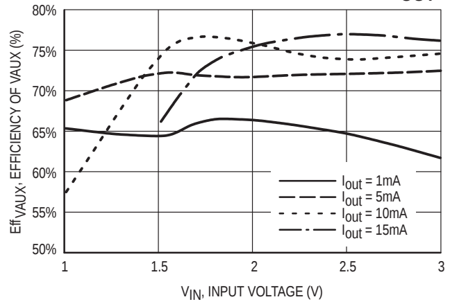
Figure 11. Efficiency of VAUX versus Input Voltage (VAUX = 20 V, L2 = 33 \mu H, Various I_{OUT} )
