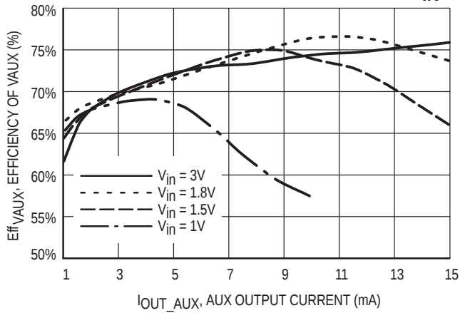
Figure 10. Efficiency of VAUX versus Output Current (VAUX = 20 V, L2 = 33 \mu H, Various V_{IN} )
