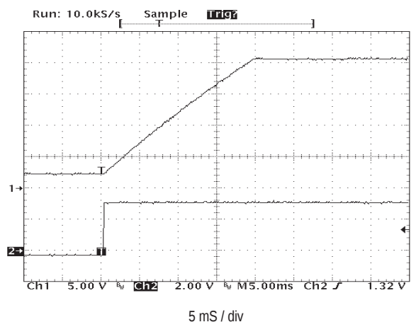
Figure 19. VAUX Startup
