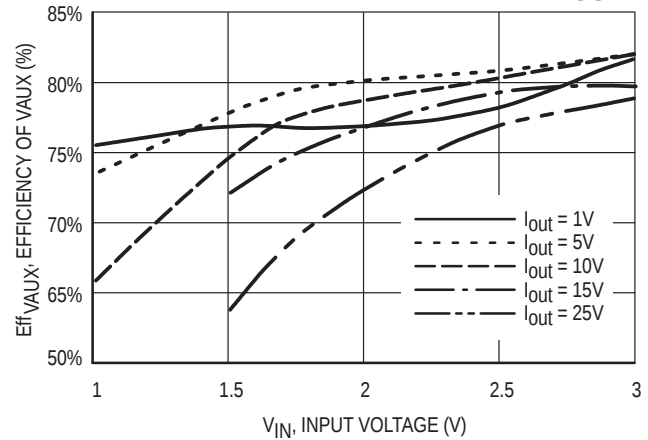
Figure 13. Efficiency of VAUX versus Input Voltage (VAUX = 5 V, L2 = 82 \mu H, Various I_{OUT} )
