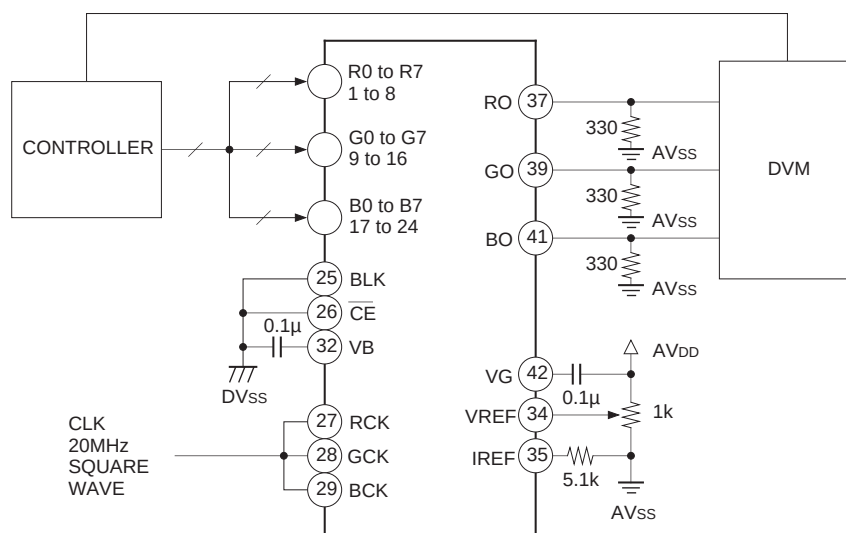
DC Characteristics Measurement Circuit
