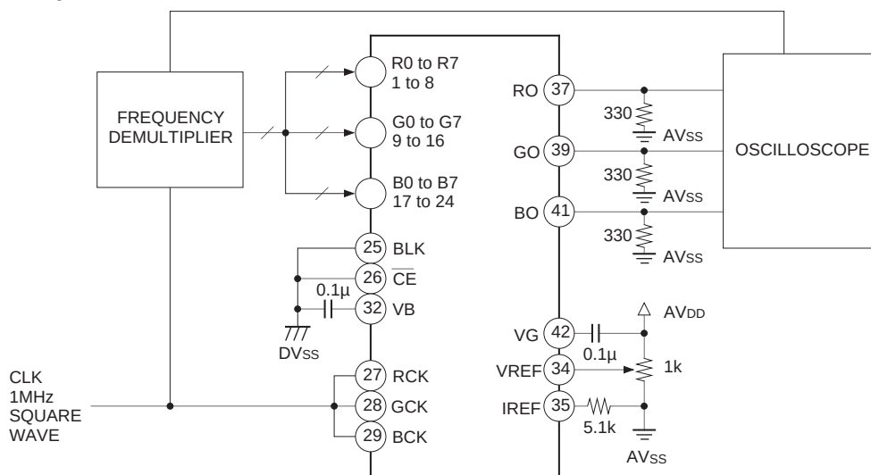
Propagation Delay Time Measurement Circuit
