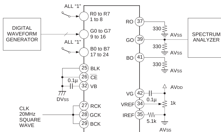
SNR Measurement Circuit
