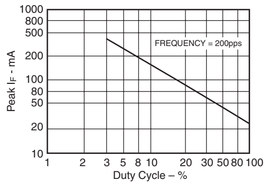
Fig. 1D. Max Peak Current vs. Duty Cycle
