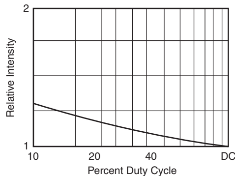
Fig. 3E. Relative Luminous Intensity vs. Duty Cycle
