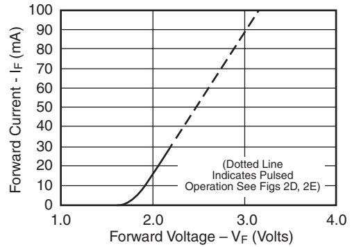
Fig. 2B. Forward Current vs. Forward Voltage
