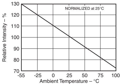
Fig. 2C. Relative Luminous Intensity vs. Temperature (See Note 2)
