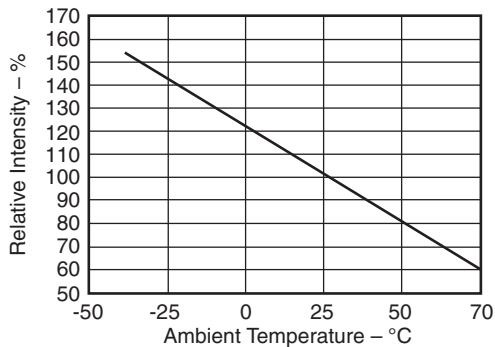
Fig. 3C. Relative Luminous Intensity vs. Temperature (See Note 2)
