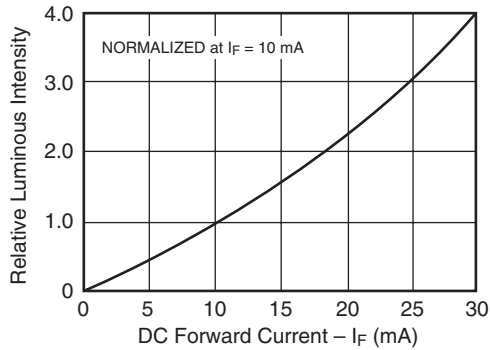
Fig. 4A. Relative Luminous Intensity vs. Forward Current
