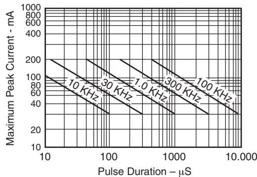
Fig. 2E. Maximum Peak Current vs. Pulse Duration
