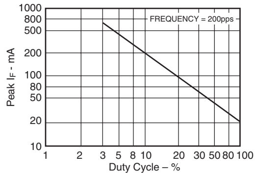
Fig. 3D. Max Peak Current vs. Duty Cycle
