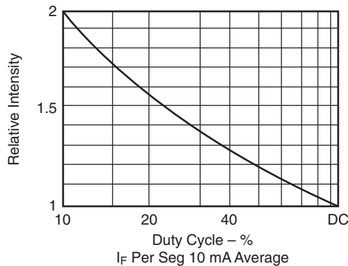
Fig. 4E. Relative Luminous Intensity vs. Duty Cycle
