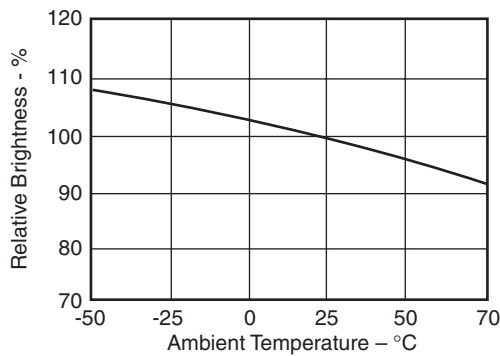
Fig. 1C. Relative Luminous Intensity vs. Temperature (See Note 2)
