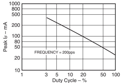
Fig. 4D. Maximum Peak Current vs. Duty Cycle
