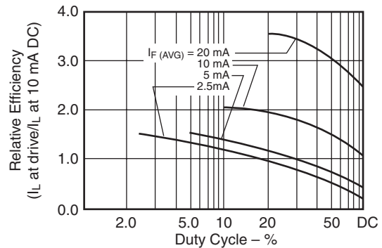
Fig. 2D. Relative Efficiency vs. Duty Cycle
