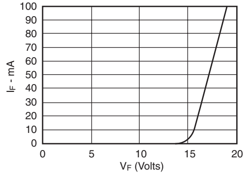
Fig. 3B. Forward Current vs. Forward Voltage
