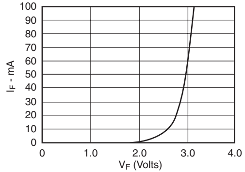
Fig. 1B. Forward Current vs. Forward Voltage
