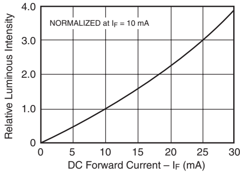
Fig. 3A. Relative Luminous Intensity vs. DC Forward Current
