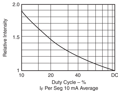
Fig. 1E. Relative Luminous Intensity vs. Duty Cycle
