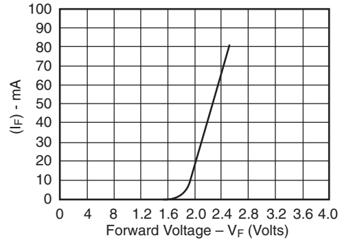
Fig. 4B. Forward Current vs. Forward Voltage
