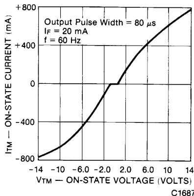
Fig. 2. On-State Characteristics
