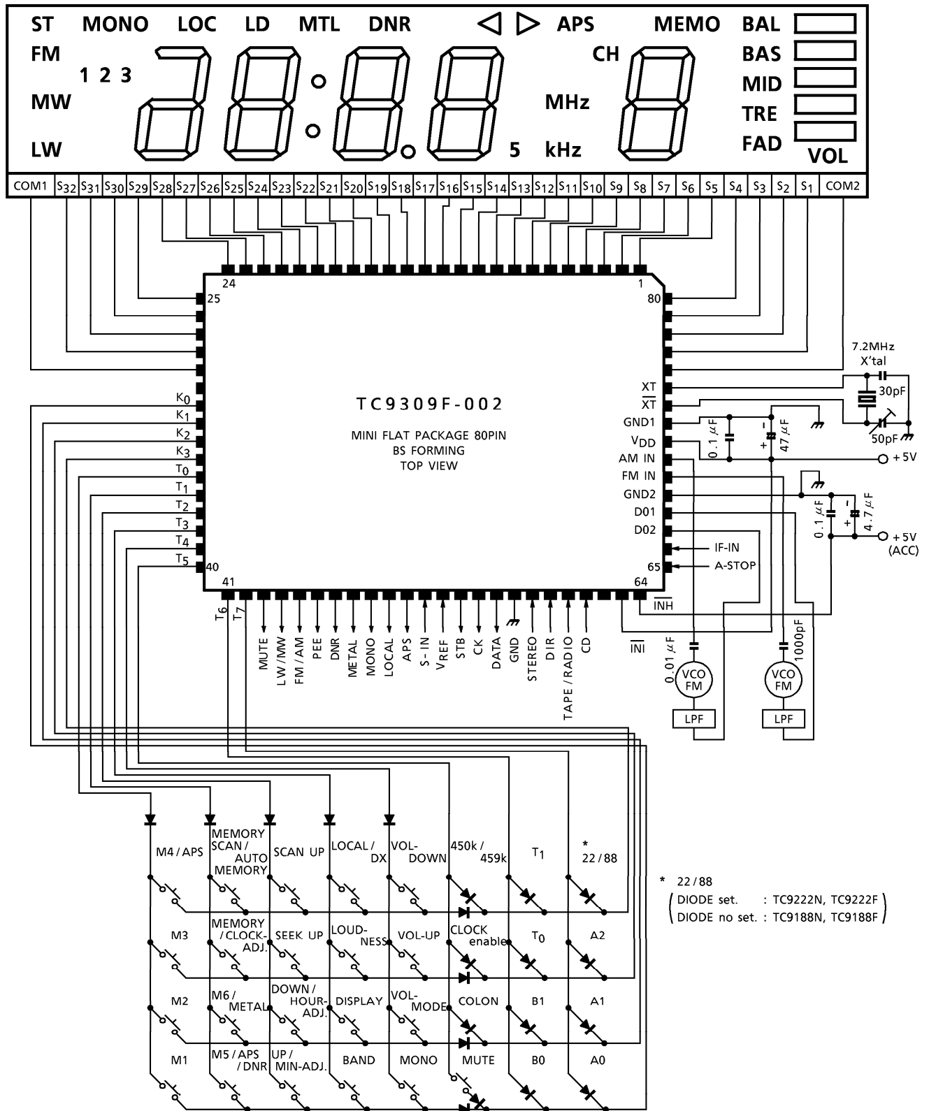
TC9309F-002 Layout
