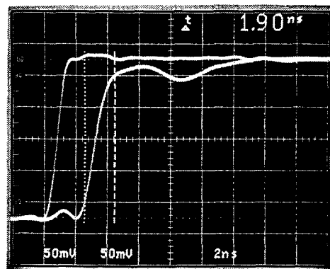
A_V = +1, \text{SMALL SIGNAL RISE TIME, WITH FET PROBES} LT1190 - TPC24
