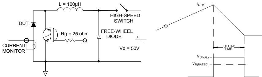
Fig. 11 - Avalanche Test Circuit and Waveforms
