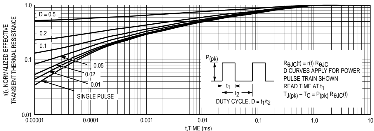
Figure 13. Thermal Response
