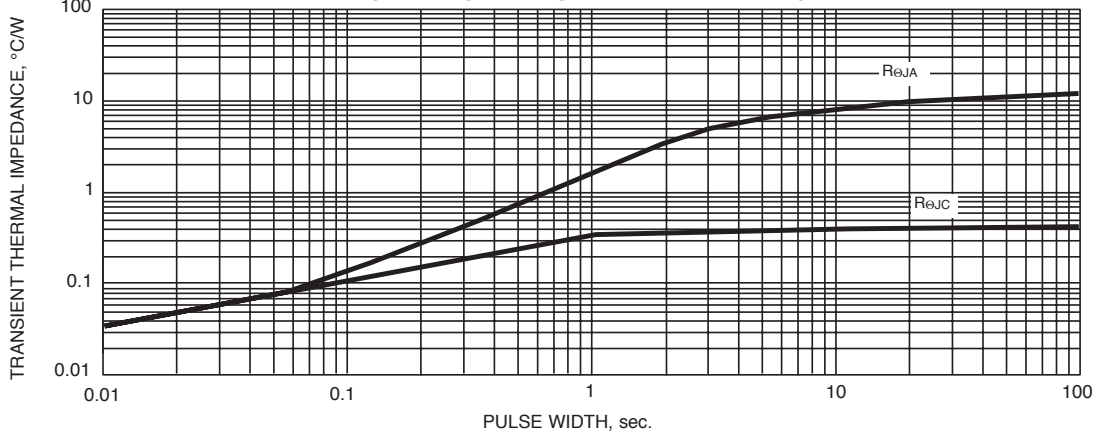
FIG. 7 - TYPICAL TRANSIENT THERMAL IMPEDANCE
