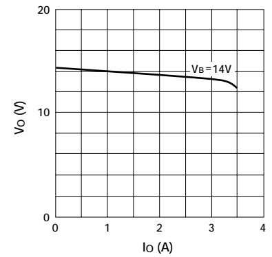
■ Overcurrent Protection Characteristics (Ta=115°C)
