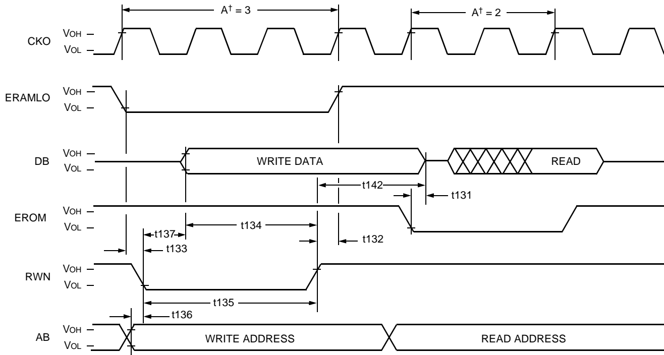
Figure 37. External Memory Data Write Timing Diagram (DENB2 = 0, DENB1 = 0, DENB0 = 0)
