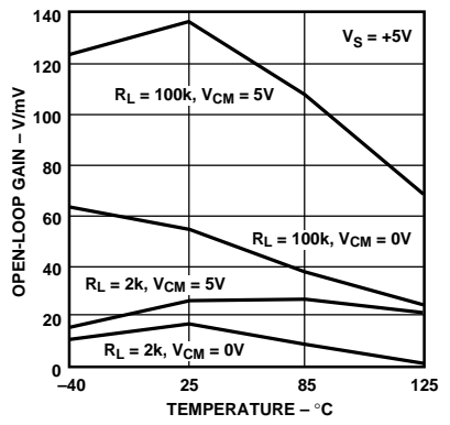
Figure 28. Open-Loop Gain vs. Temperature, V_S = +5\text{ V}
