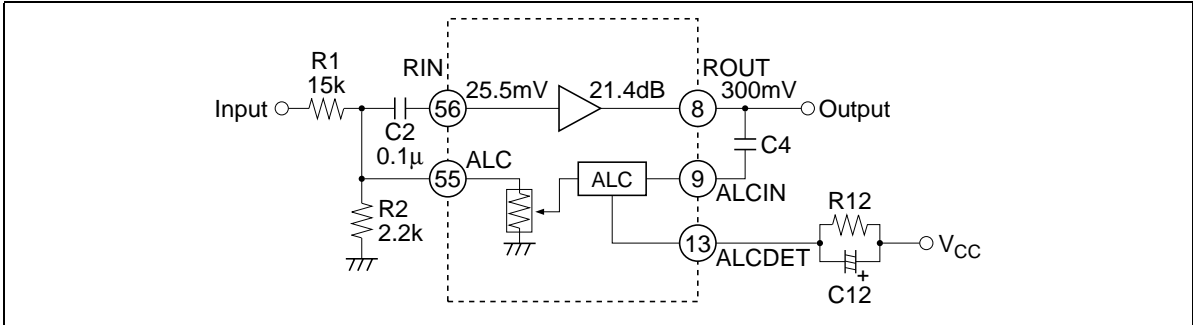
Figure 12 ALC Block Diagram
