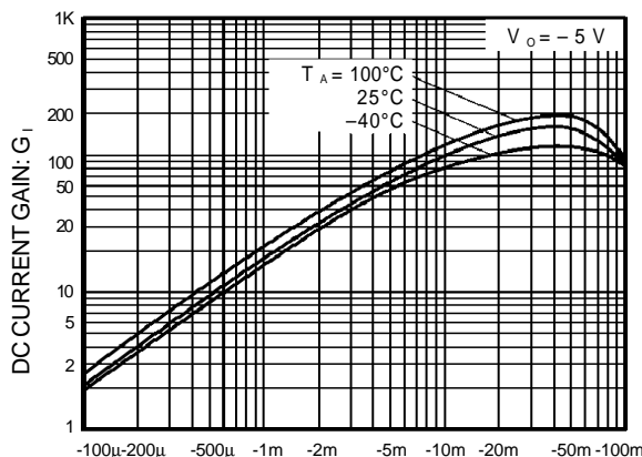
Figure 3. DC current gain vs.output current
