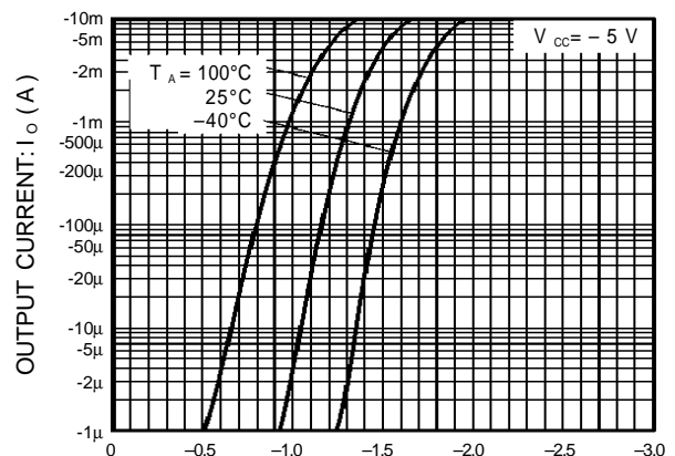
Figure 2. Output current vs.input voltage (OFF characteristics)
