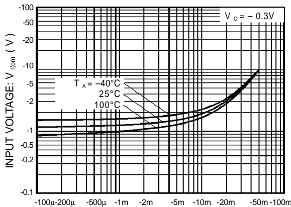
Figure 1. Input voltage vs.output current (ON characteristics)
