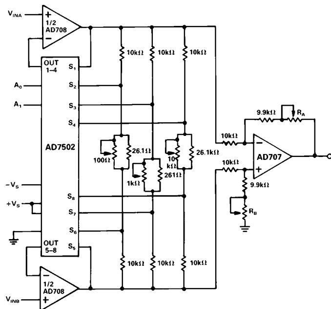
Figure 28. Precision PGA
