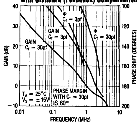
Gain, Phase Shift vs Frequency with Standard (Feedback) Compensation
