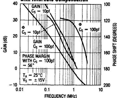
Gain, Phase Shift vs Frequency with Alternate Compensation
