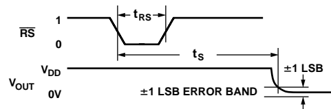
Figure 1c. Reset Timing Diagram
